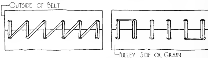
FIG. 220. WIRE LACING.
